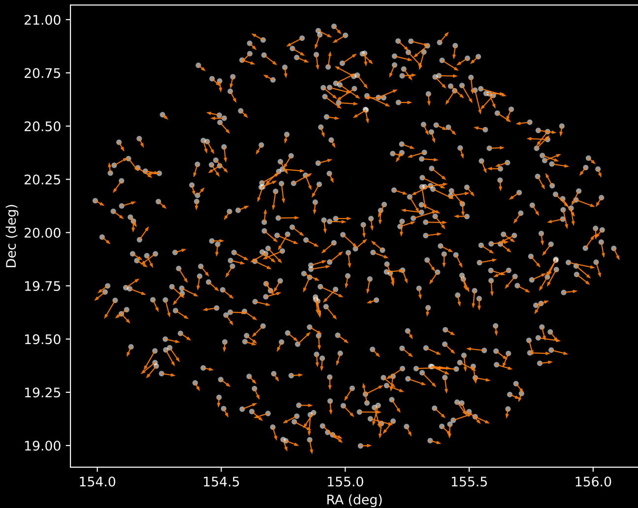
GALAH DR4 Cluster 2 Proper Motion Vectors (n=413)
