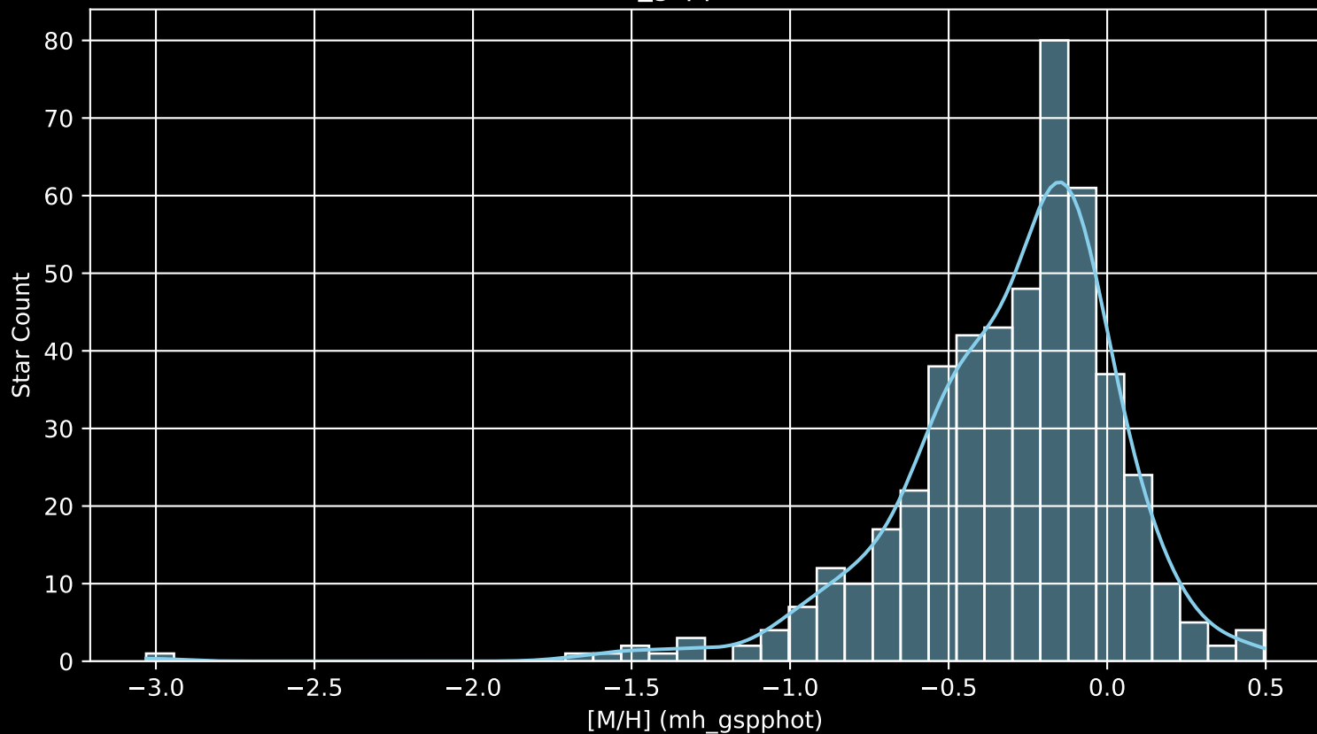
GALAH DR4 Field: [6598] [M/H] (mh_gspphot) (n= 477)
