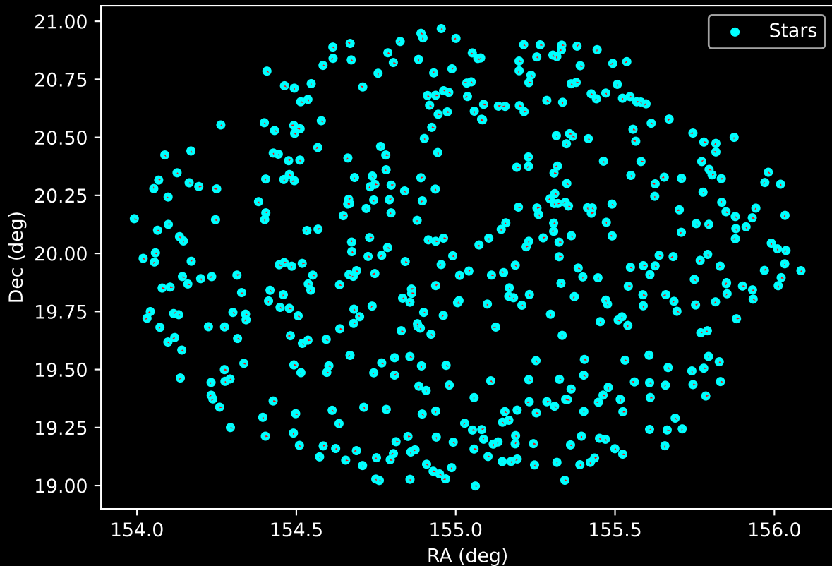
GALAH DR4 Field: [6598] Proper Motion Vectors for Gaia Star Field (n= 478)
