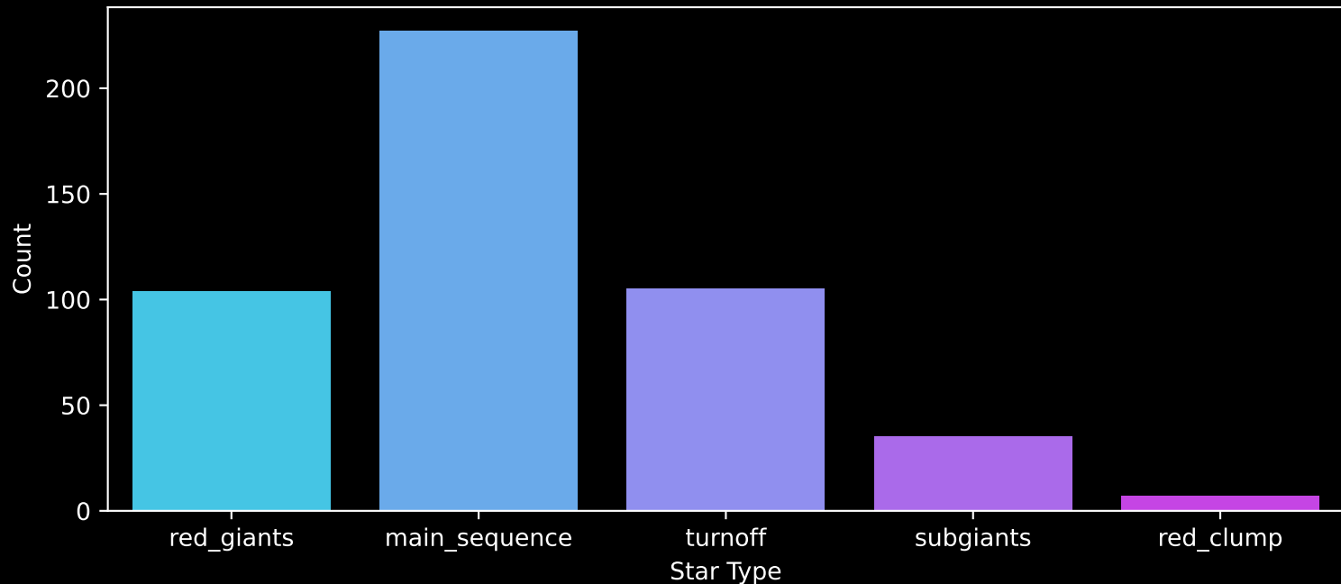
GALAH DR4 Field: [6598] Count plot of Star Type
