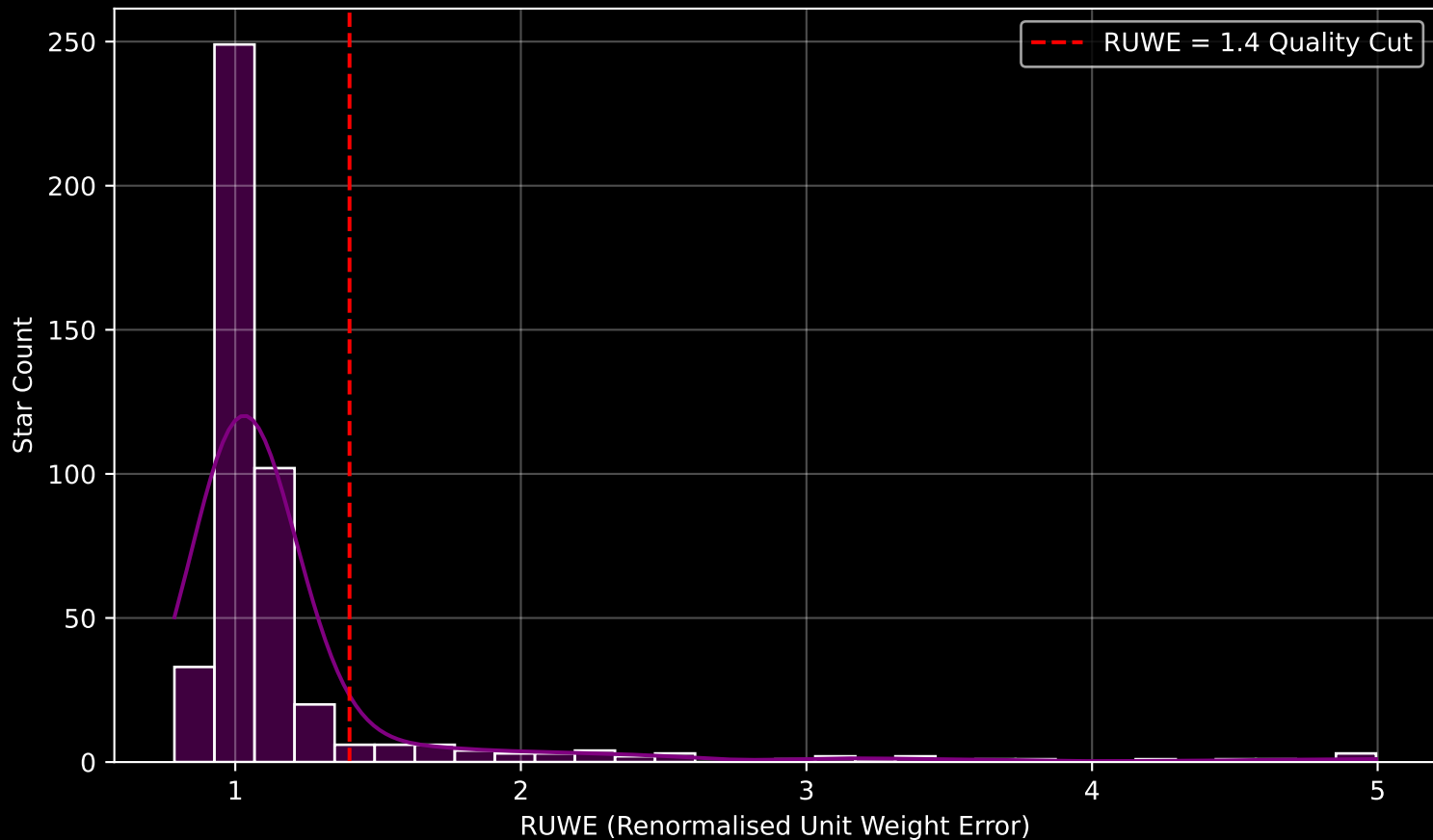
GALAH DR4 Field [6598] RUWE Distribution (n= 455)
