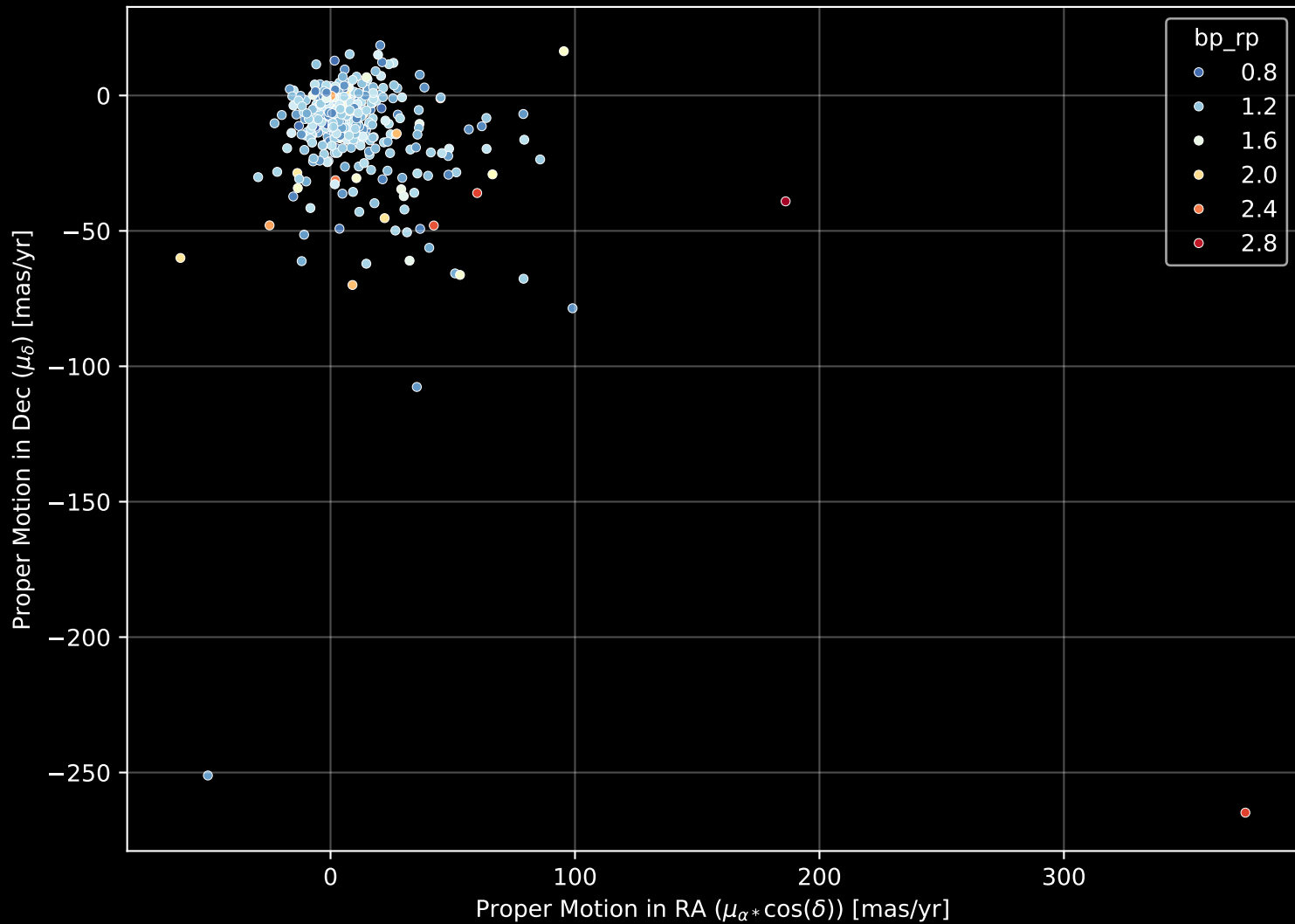
GALAH DR4 Field: [6598] Proper Motion Diagram (n= 478)
